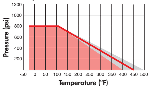
1 1/2" – 2" Valves
