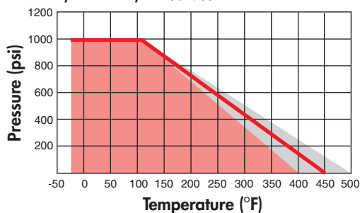
1/4" – 1 1/4" Valves
